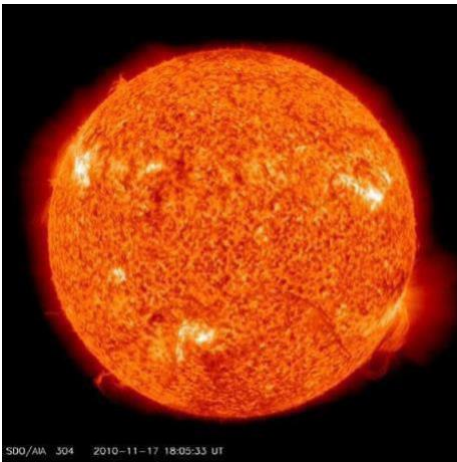
The Sun - Credit: NASA
