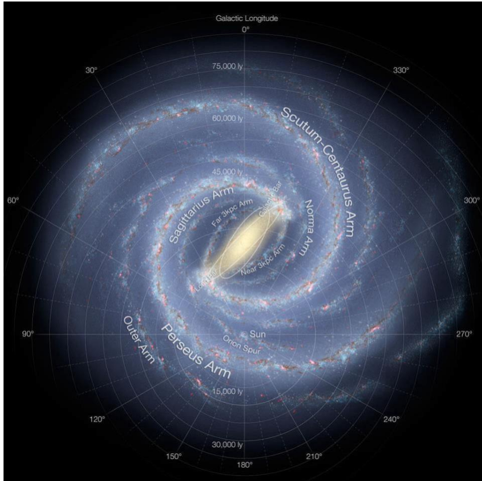
Artist's conception of the spiral structure of the Milky Way with two major stellar arms and a bar. Credit: NASA/JPL-Caltech/ESO/R. Hurt
