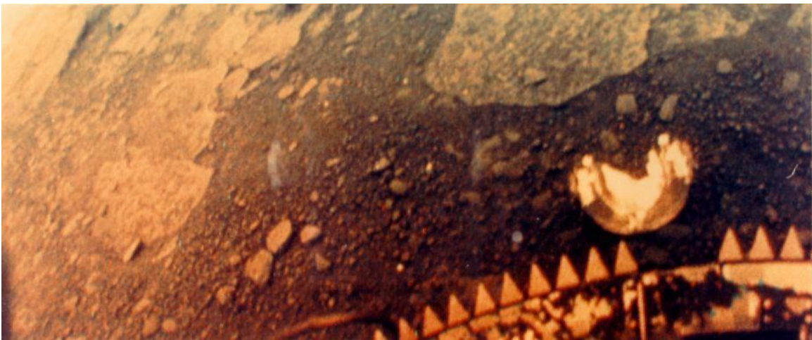
Surface photograph from the Soviet Venera 13 spacecraft.
